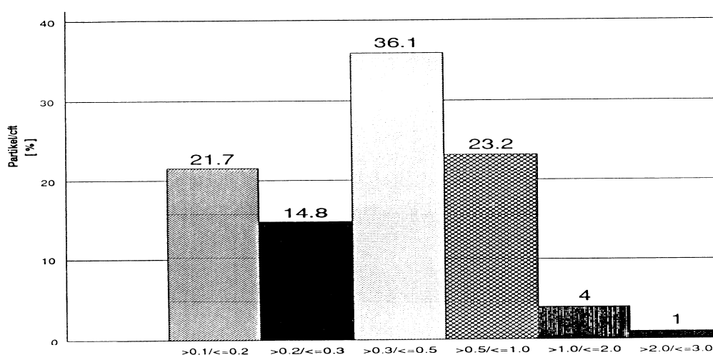
Fig. 2: Relative frequency of the Classes of Particle Size (size in \mu m)
